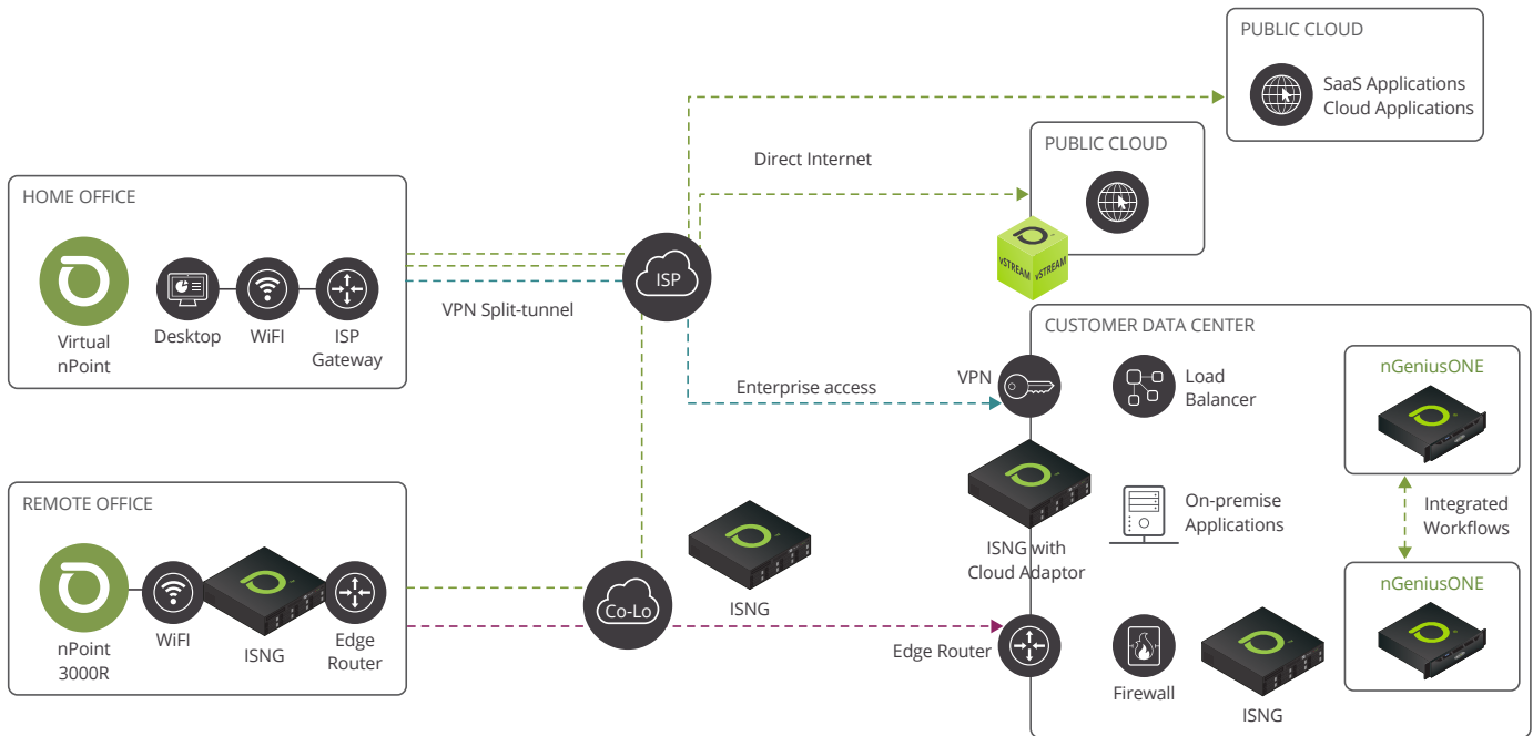
Figure 2: Comprehensive visibility comes from the unique combination of strategically deployed InfiniStreamNG appliances with Cloud Adaptor at the Network Edges, and vSTREAM appliances in Data Center / Cloud Service Edges, along with nPoint devices at end-use sites. This enables organizations to pinpoint the true root cause of problems from the remote location network, user’s ISP, VPN or corporate infrastructure, to the data center or public cloud, or any other domain the transaction depends on.
