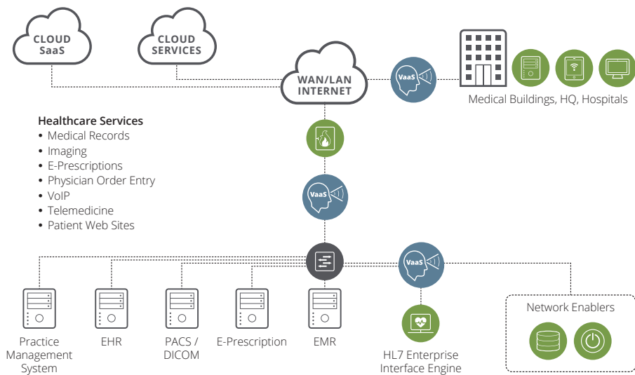
Figure 1: EHR Management Systems - complex web of network, infrastructure, applications, standards and protocols in a hybrid cloud environment.
