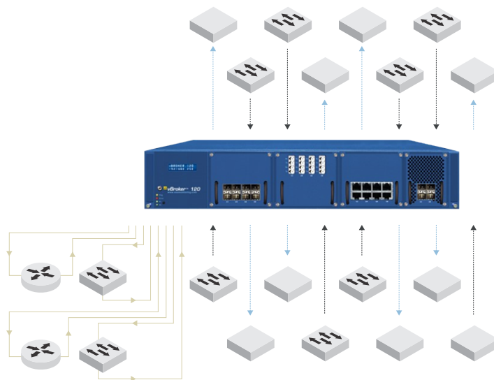
Figure 1: Backbone of Large Scale Monitoring Infrastructure in the Data Center.
