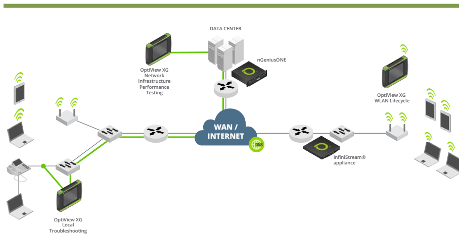
Figure 1: OptiView XG is a portable wireless tablet designed to troubleshoot wired and wireless site networks.
